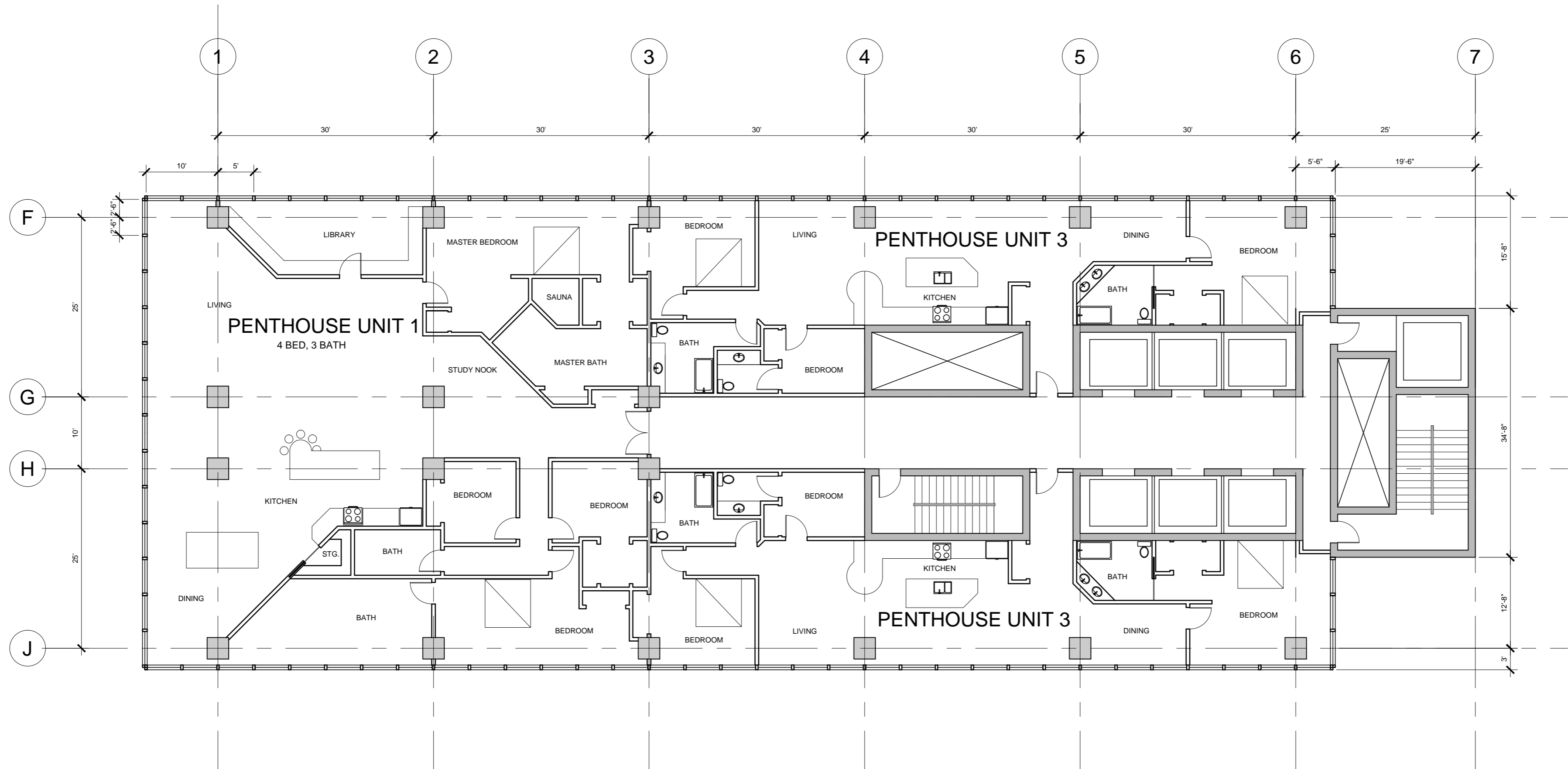
1 PENTHOUSE PLAN A9 1/8"=1'-0"
